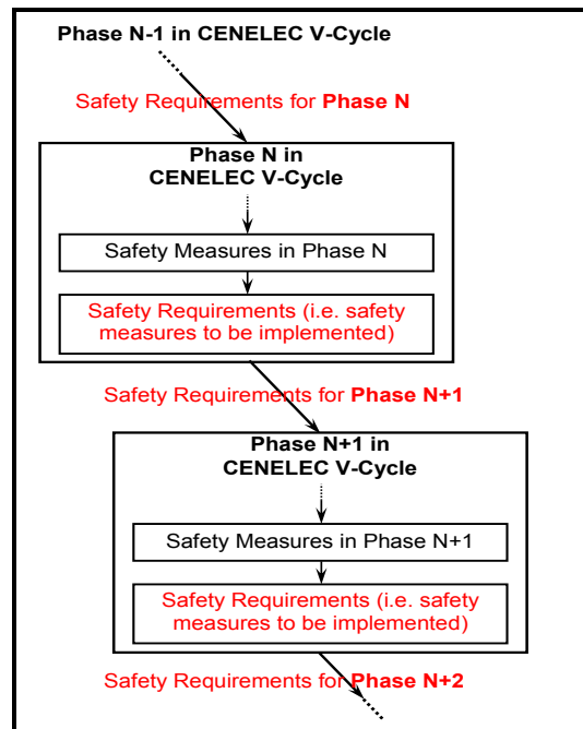
Figure 11 : Derivation of the safety requirements for lower level phases.
