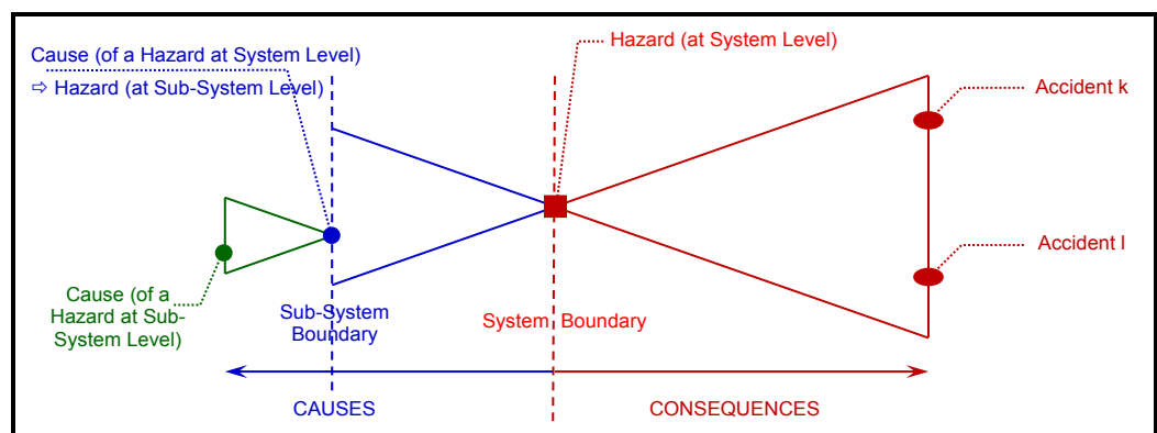
Figure 10 : Figure A.4 of EN 50 129: Definition of hazards with respect to the system boundary.
