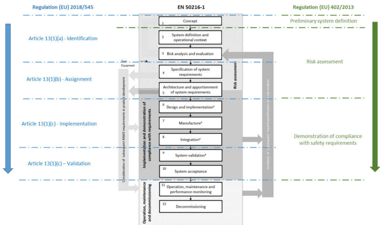
Figure 4: requirements capture in Regulation (EU) 2018/545 vs CSM RA process and system life cycle in EN 50126-1
